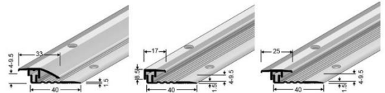
PPS Champion Star 4-9.5 mm
