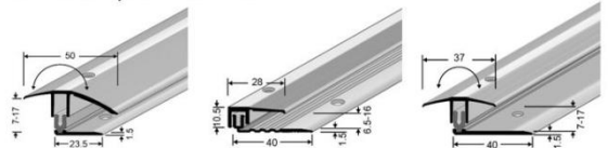
PPS Champion Flex 7-17 mm
